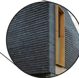
BRICK VENEER DETAILING
